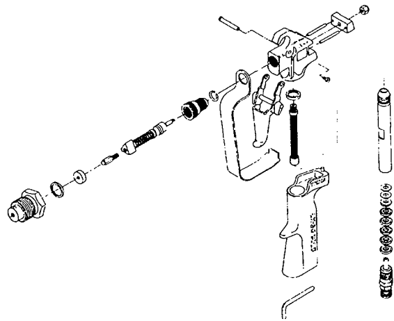
Figure 9 -- For more detail, part number information and assembly drawings at larger scale, please see the LX 80 Gold Professional Airless Gun Owner's Manual (#313-687).
