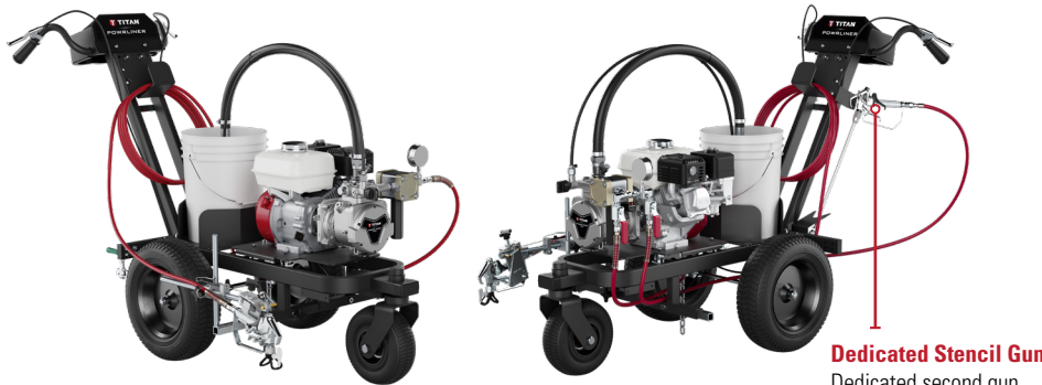
PowrLiner 3500S: Includes RX-80 gun with 419 line striping tip plus dedicated RX-80 gun with 18" extension and SC-6+ 517 tip for stenciling.
